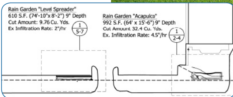
Below: Layout plan for two of the parking lot raingardens
